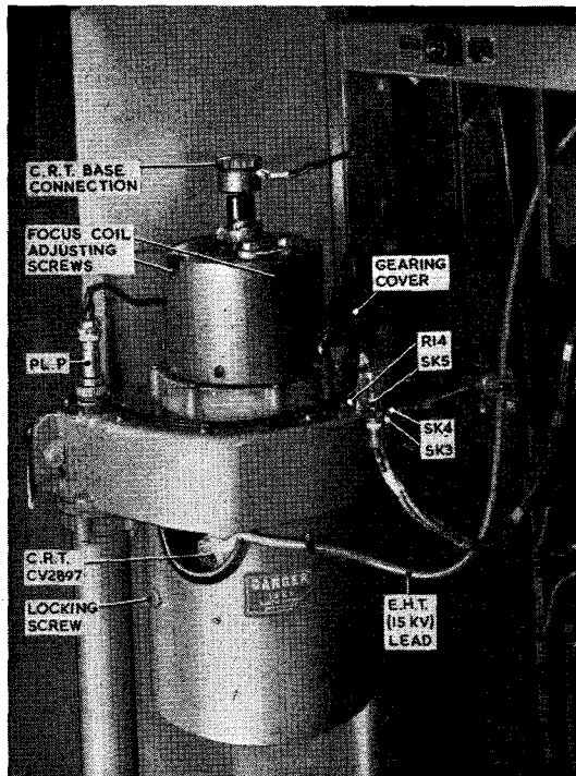
Fig. 6. Indicating unit (CRT) Type 33, upper portion
