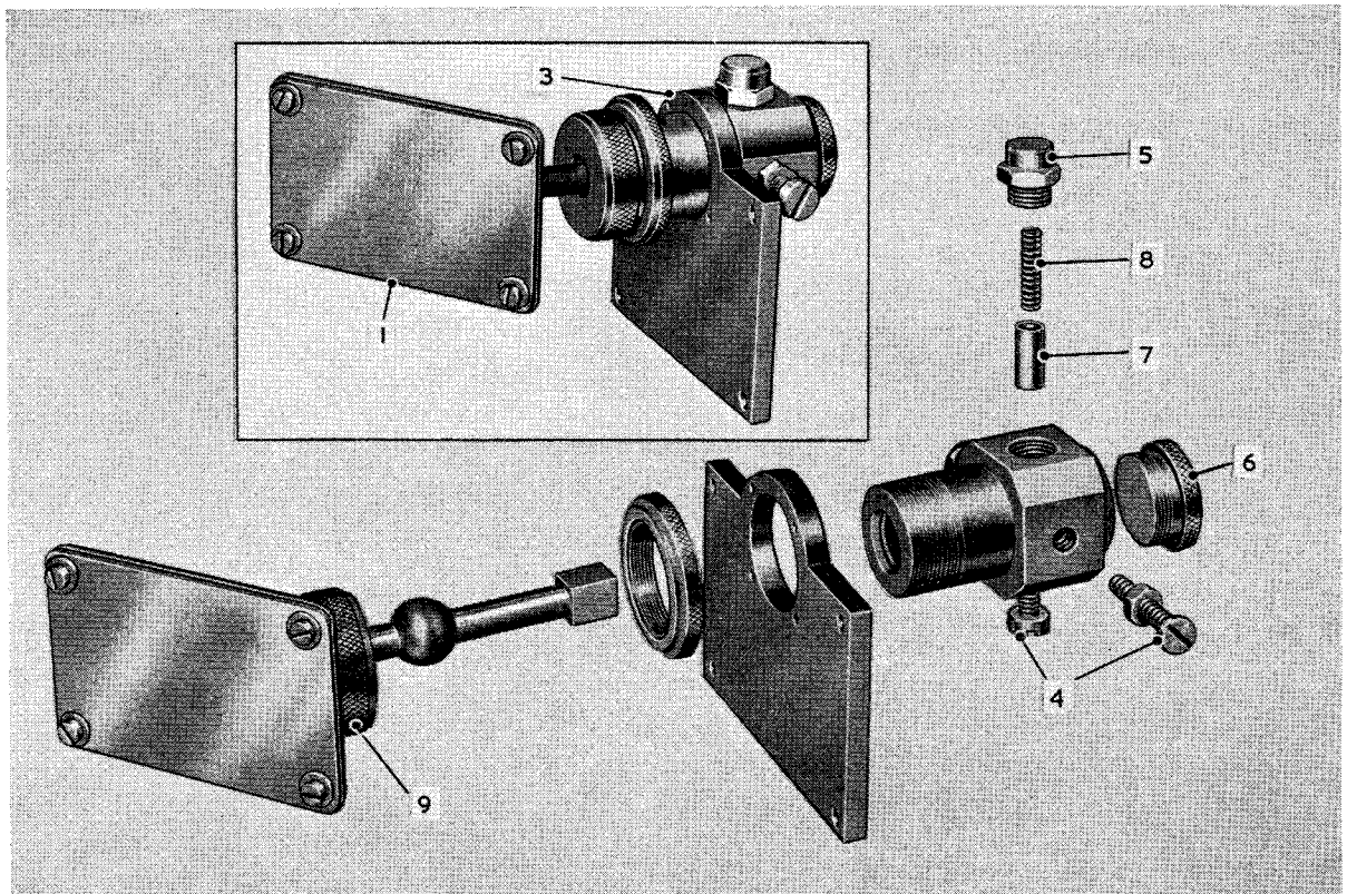
1 MIRROR 3 MIRROR ADJUSTMENT 4 ADJ. SCREW 5 CAP (TOP AND SIDE) 6 END CAP 7 PLUNGER 8 PLUNGER SPRING 9 INNER ADJUSTING RING
