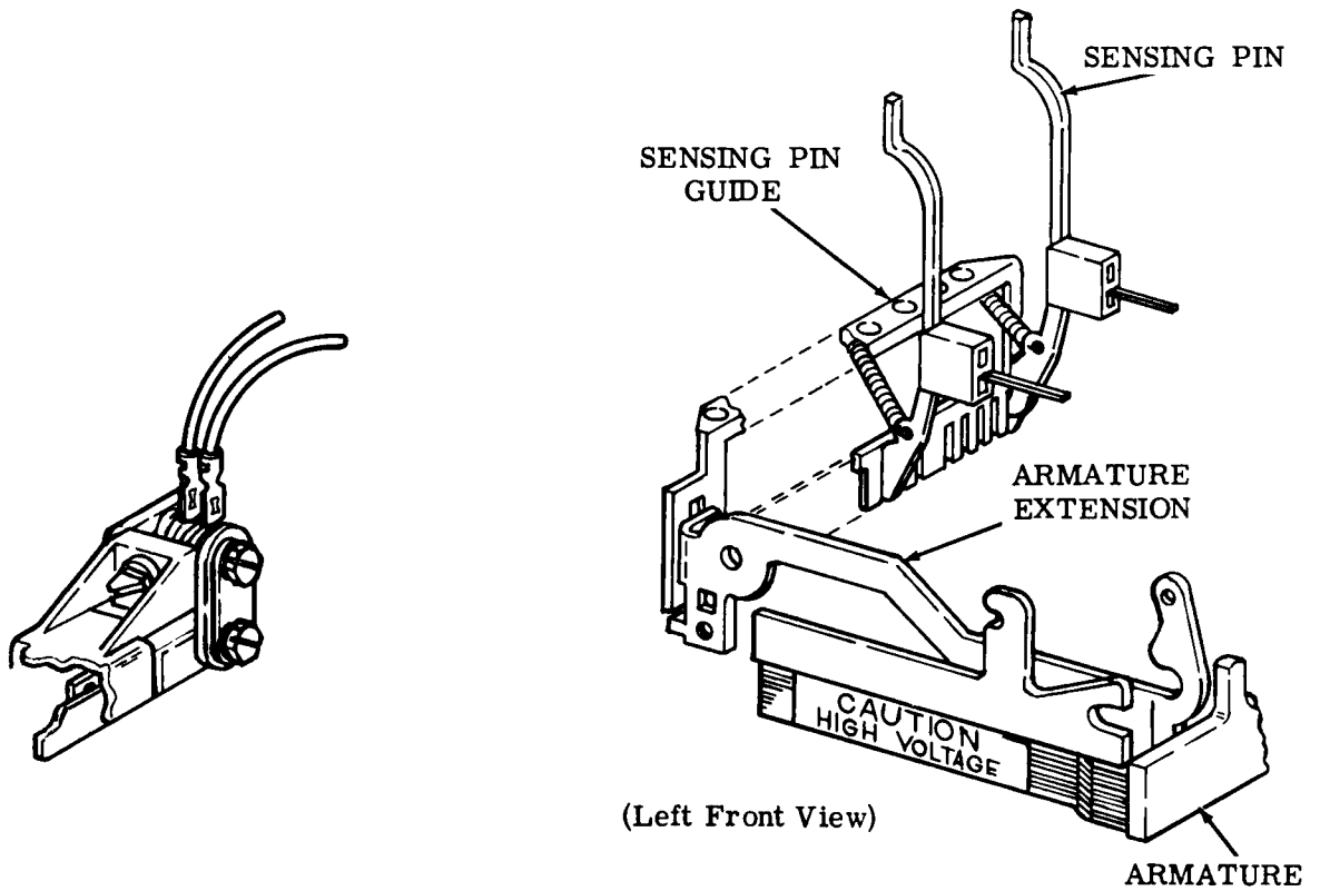
Figure 11 - Feed Magnet Contacts
