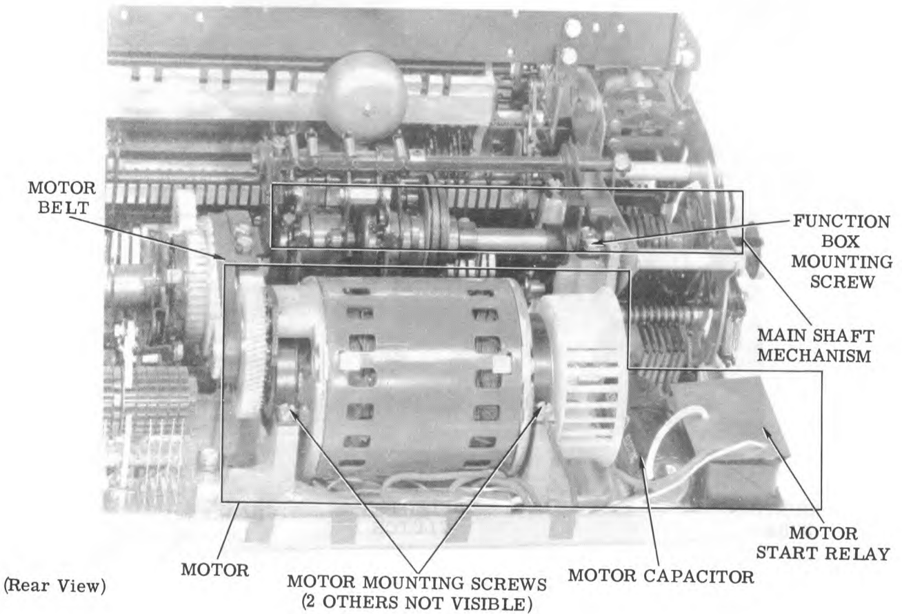
Figure 7 - Typing Unit
