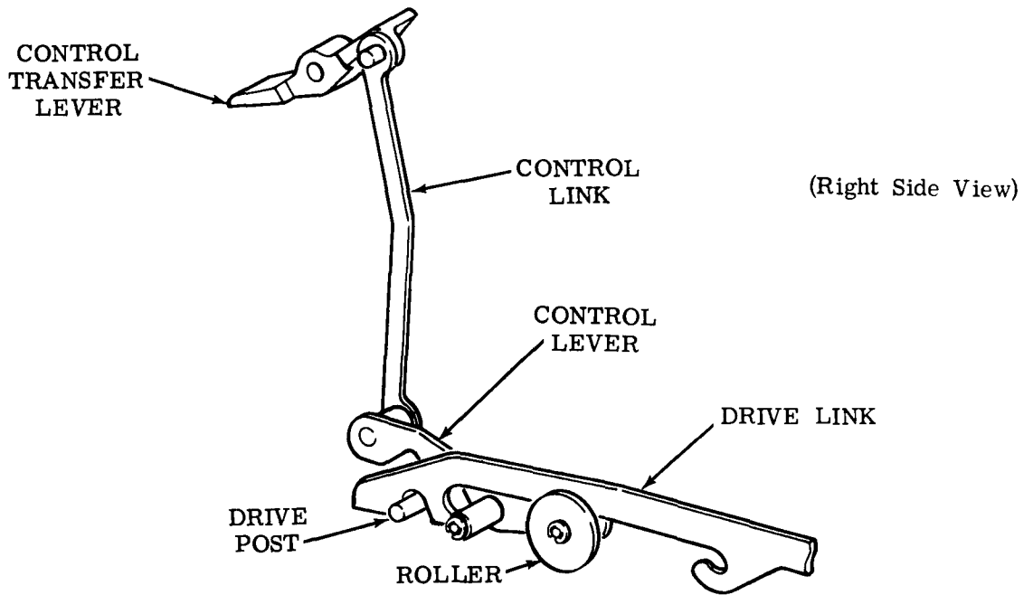
Figure 8 - ON-OFF Mechanism
