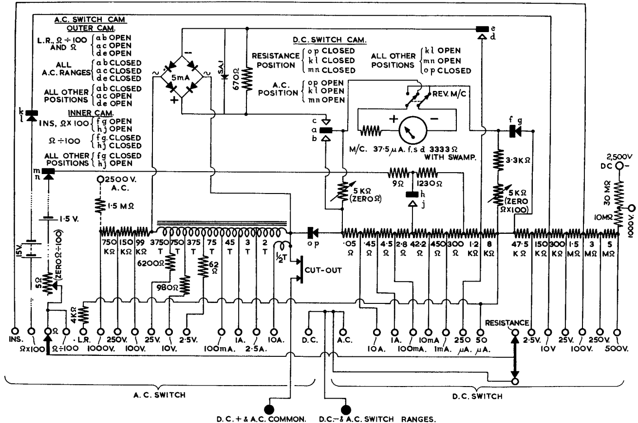
CIRCUIT DIAGRAM OF THE MODEL 8 AVOMETER MK. II
