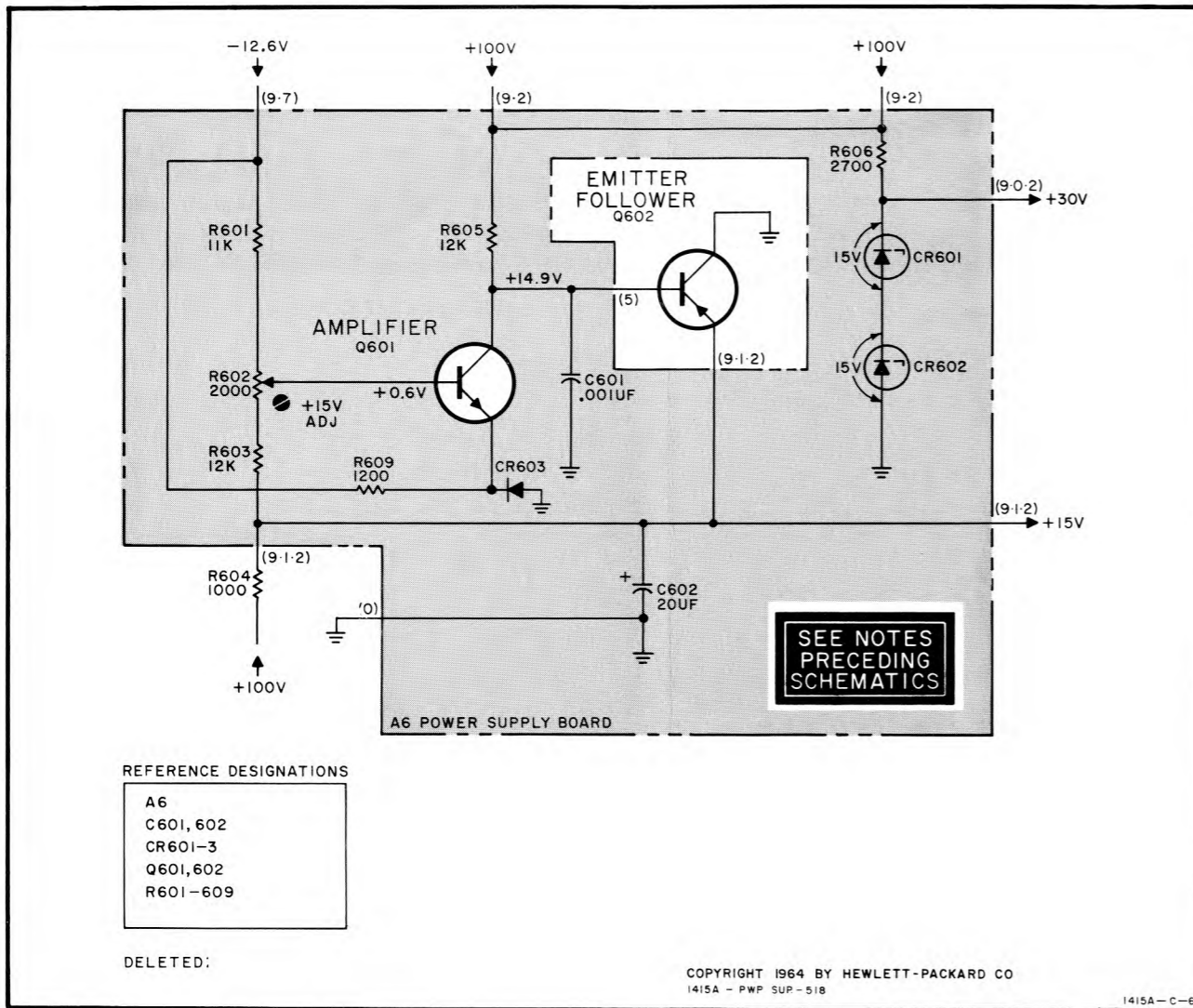
Figure 5-24. Power Supply Schematic Diagram
