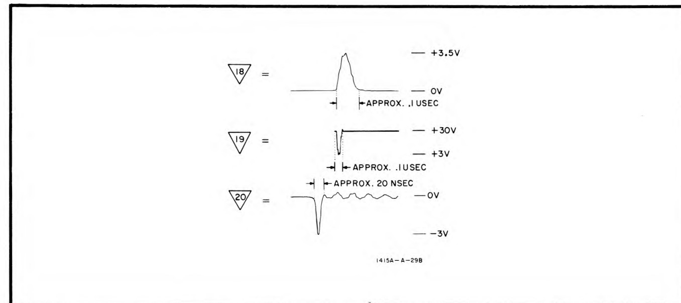
Figure 5-17. Waveforms at Test Points in Sampler Circuit
