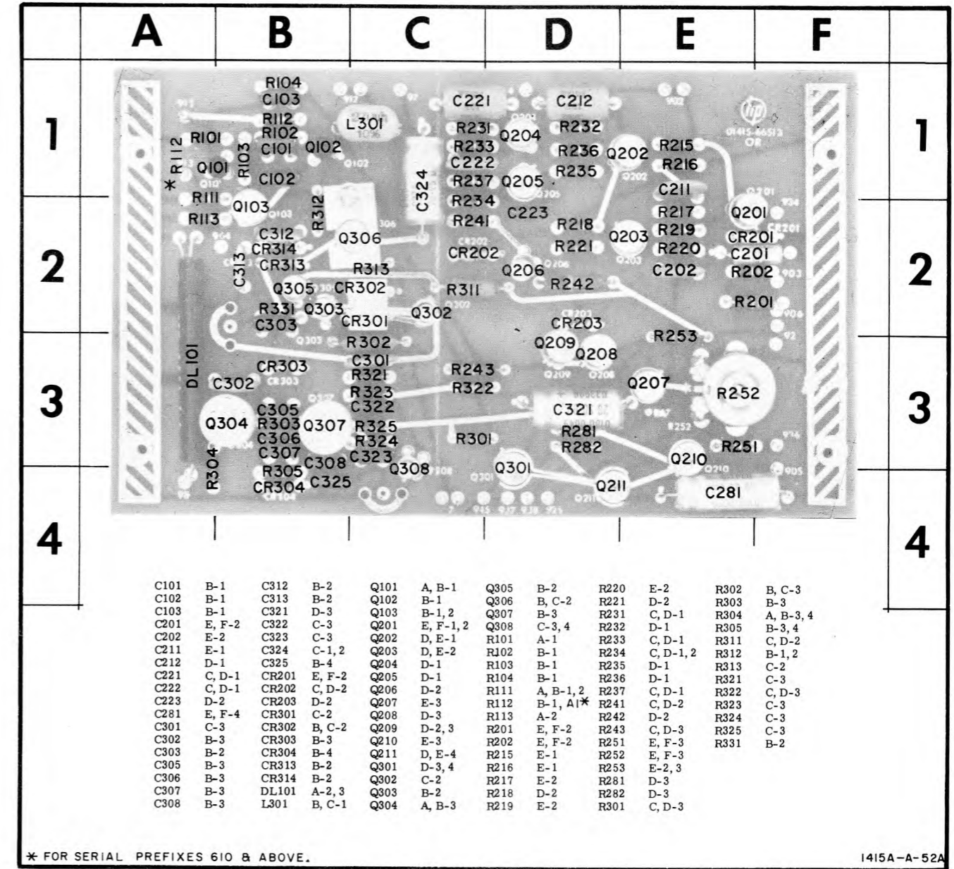
Figure 5-9. Component Locations on A1, Time Base Board
