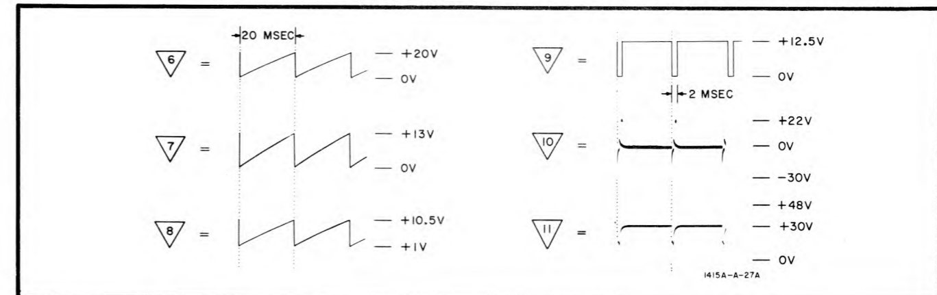
Figure 5-10. Waveforms at Test Points in Slow Ramp and Dot Comparator
