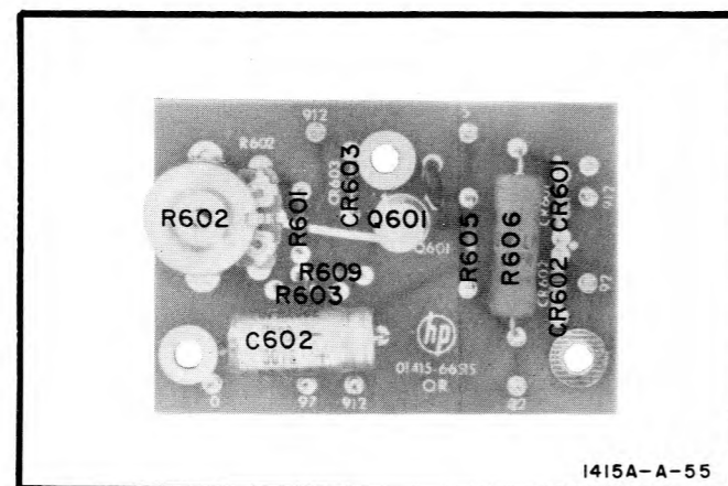
Figure 5-25. Component Locations on A6, Power Supply Board
