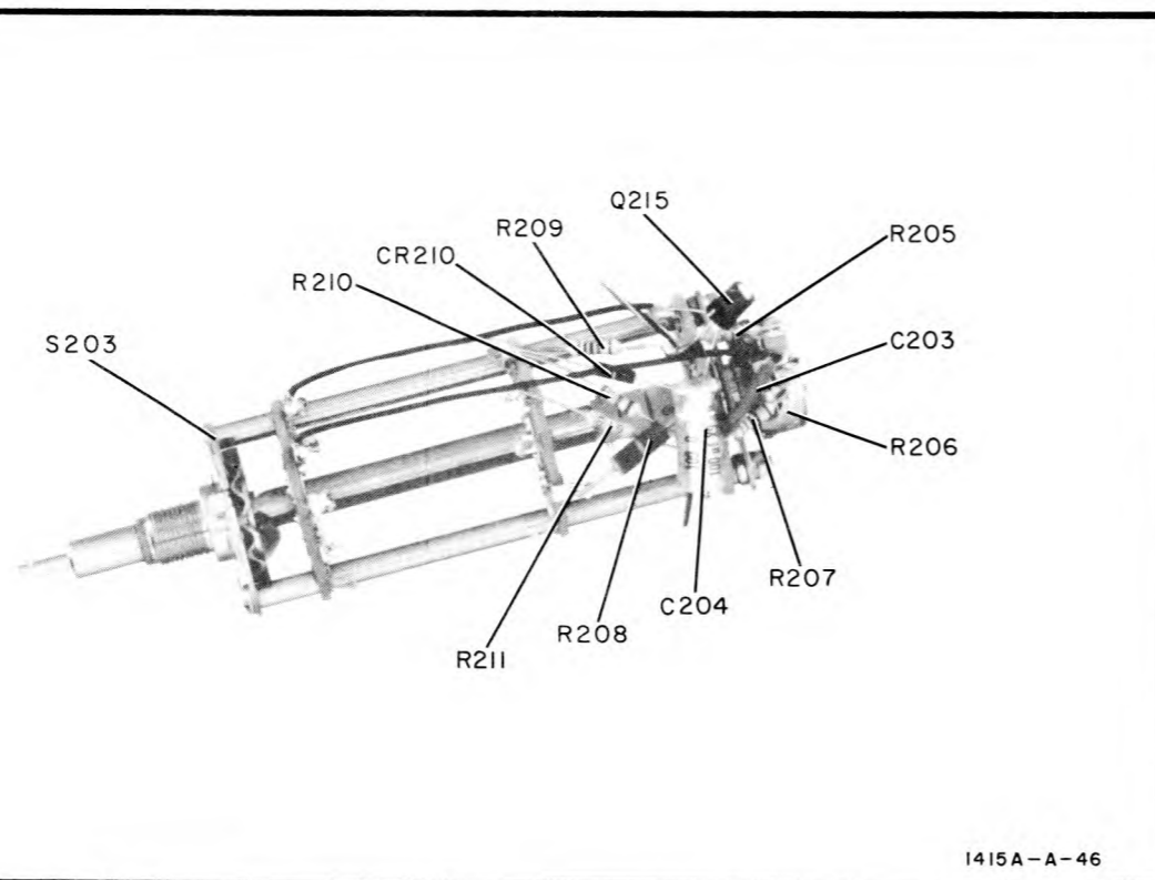
Figure 5-8. Component Locations on A13, Sweep Switch
