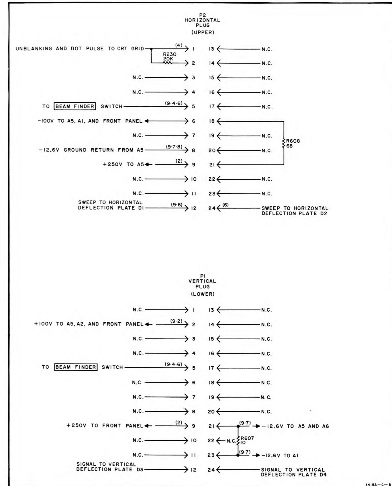
Figure 5-26. Interconnection Plugs Schematic Diagram
