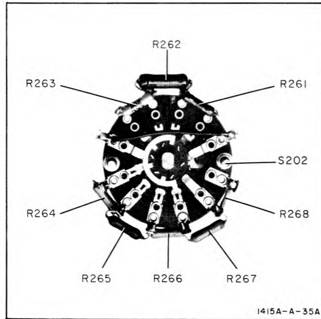
Figure 5-7. Component Locations on A10, Distance/Time Magnifier Switch
