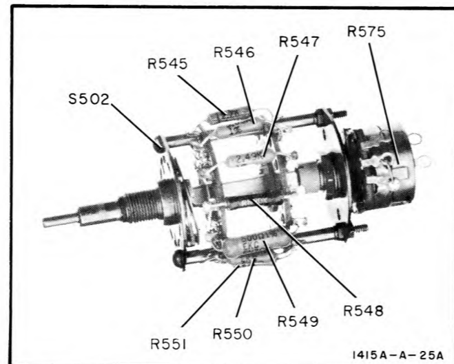
Figure 5-21. Component Locations on A8, Reflection Coefficient Switch
