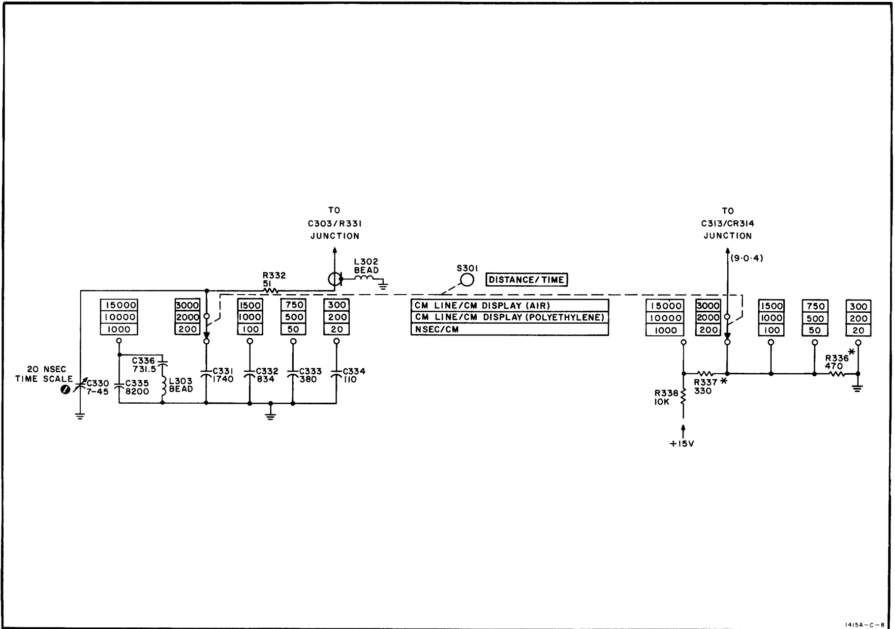
Figure IA-2. Option 14 Distance/Time Switch Schematic.
