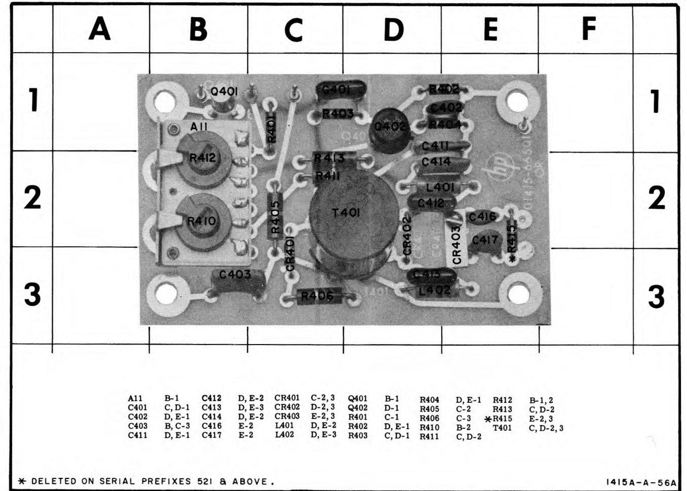
Figure 5-16. Component Locations on A3, Sampler Board
