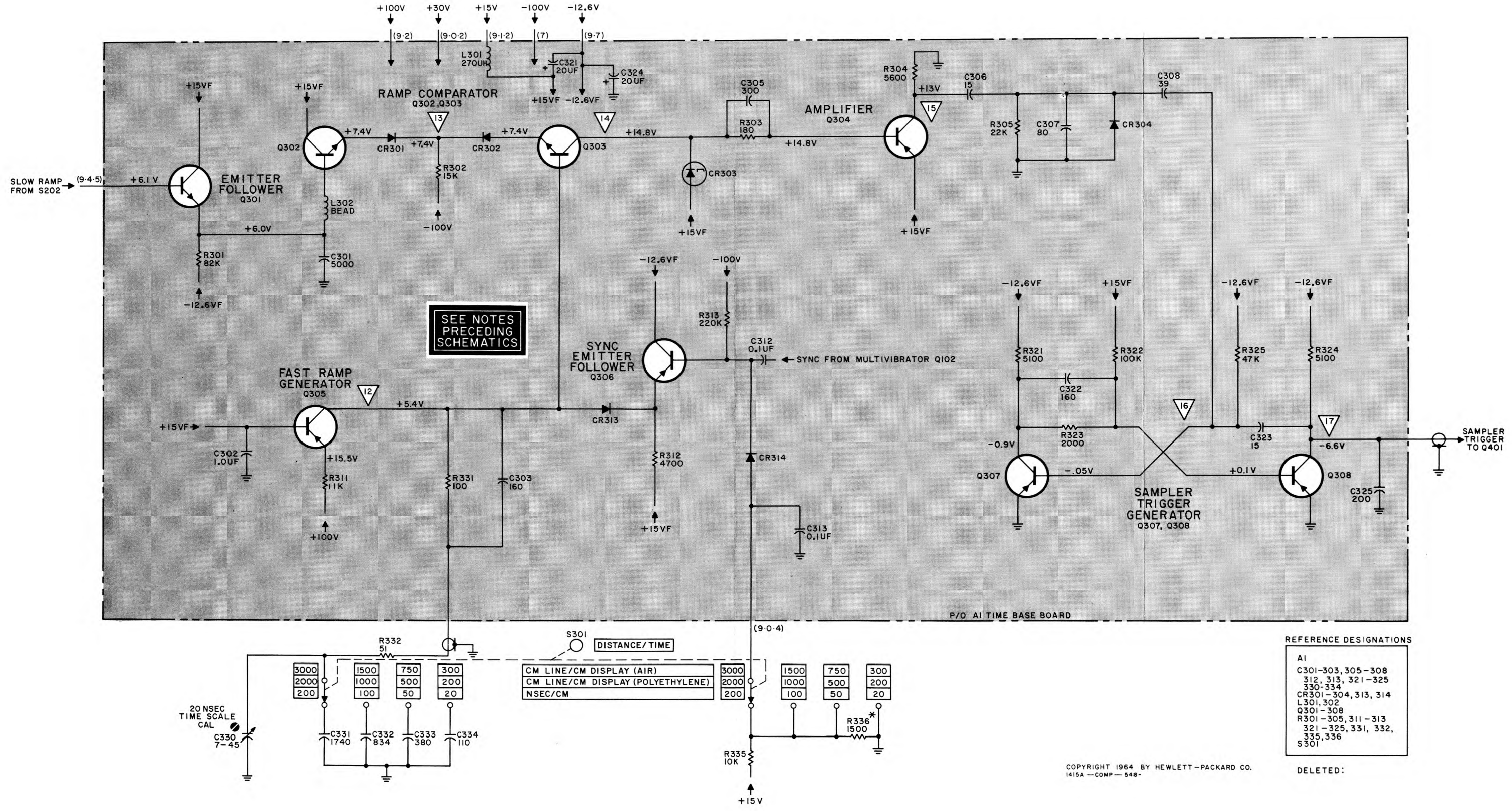
Figure 5-14. Fast Ramp and Comparator Schematic Diagram
