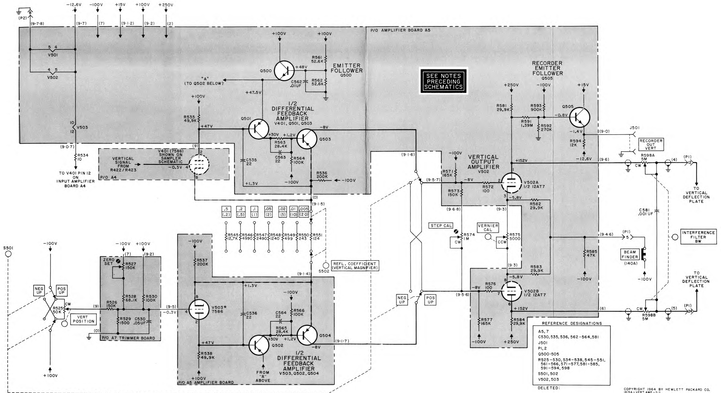
Figure 5-23. Vertical Amplifier Schematic Diagram 5-19
