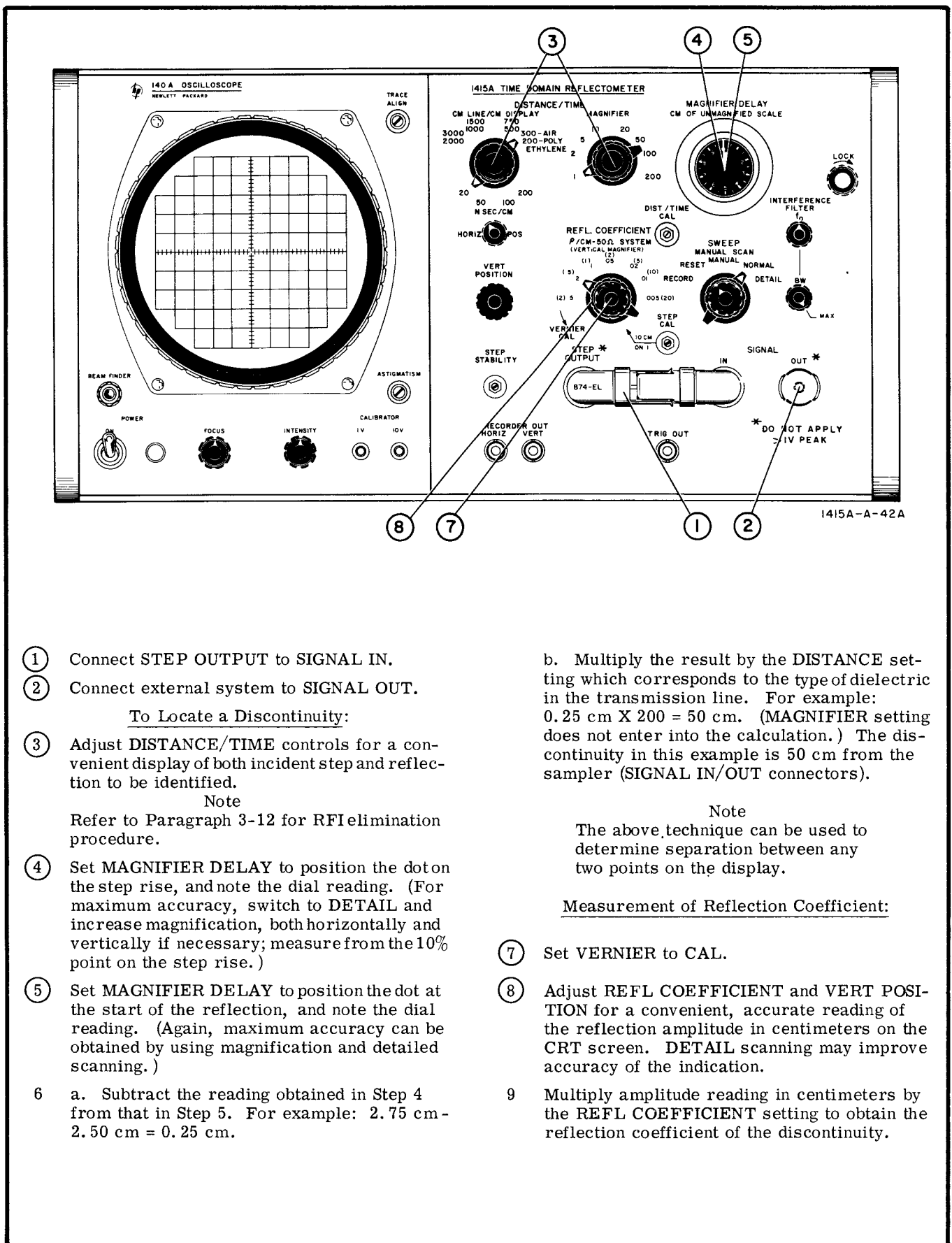
Figure 3-5. Reflection Measurements
