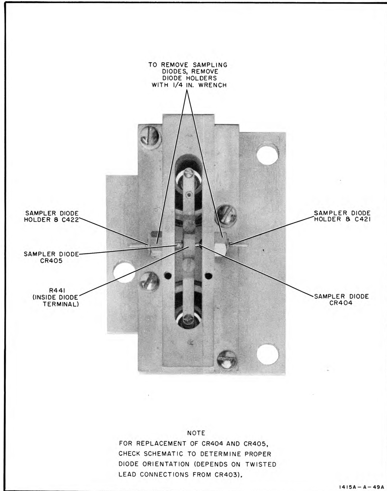
Figure 5-15. Component Locations on Sampler Block Assembly
