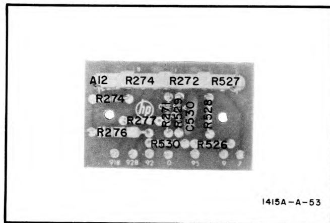
Figure 5-20. Component Locations on A7, Trimmer Board
