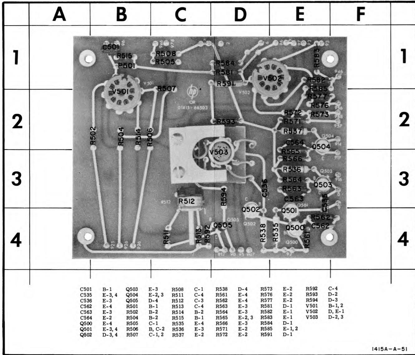
Figure 5-19. Component Locations on A5, Amplifier Board
