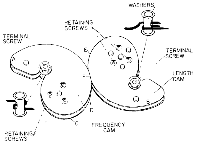
Figure 5-12. Cam Assembly
