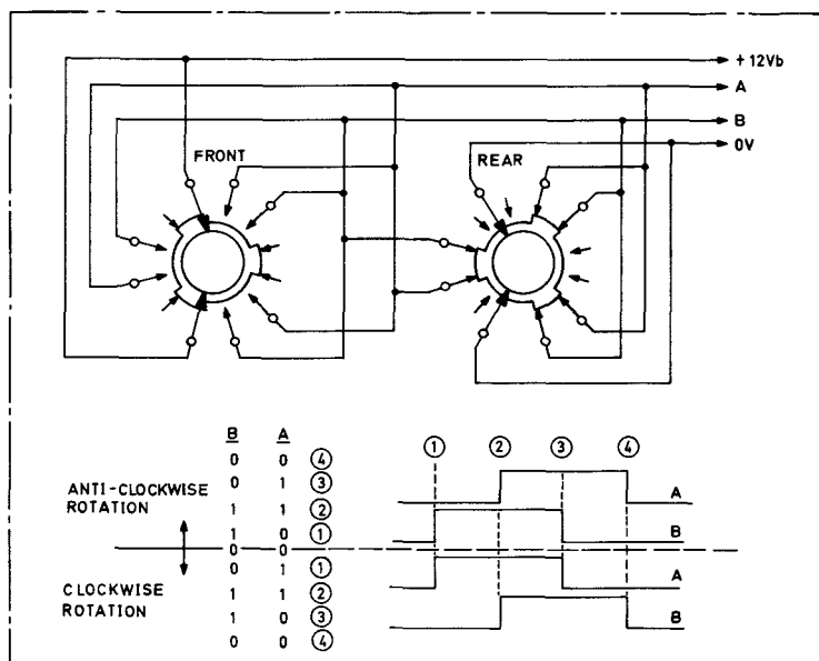
Frequency Switches : Output Waveforms
