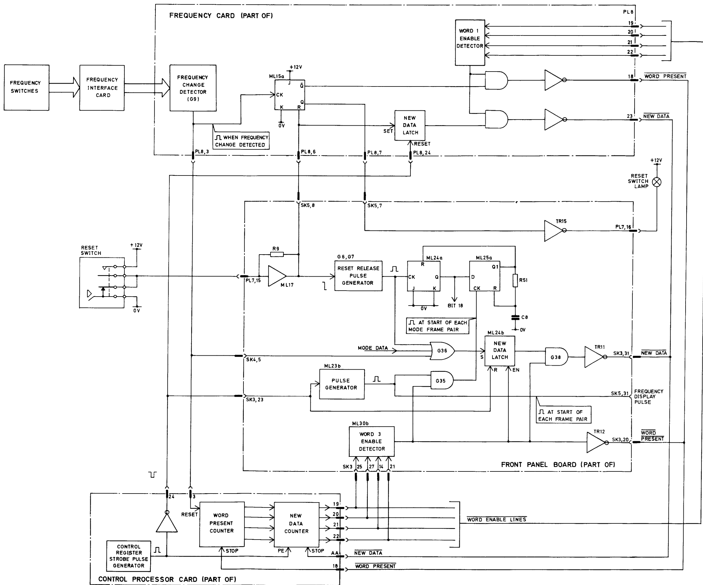
Simplified Diagram : Reset Operation
